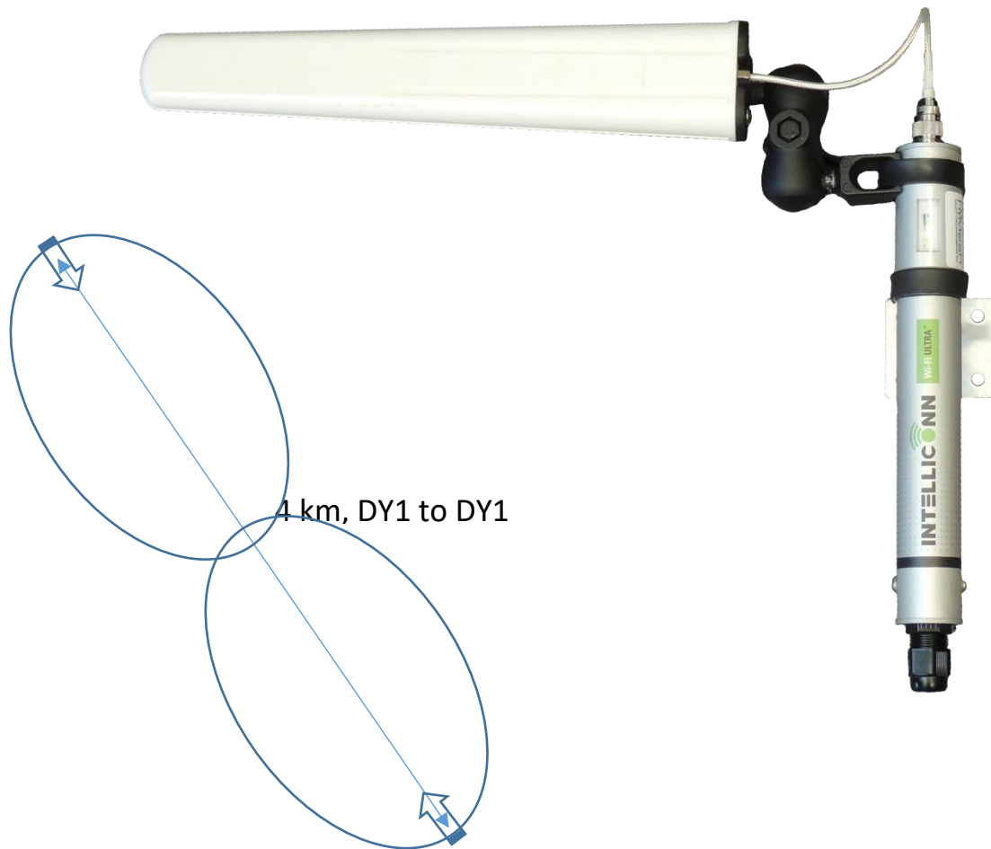
Yagi Antenna to Yagi Antenna Coverage Pattern
